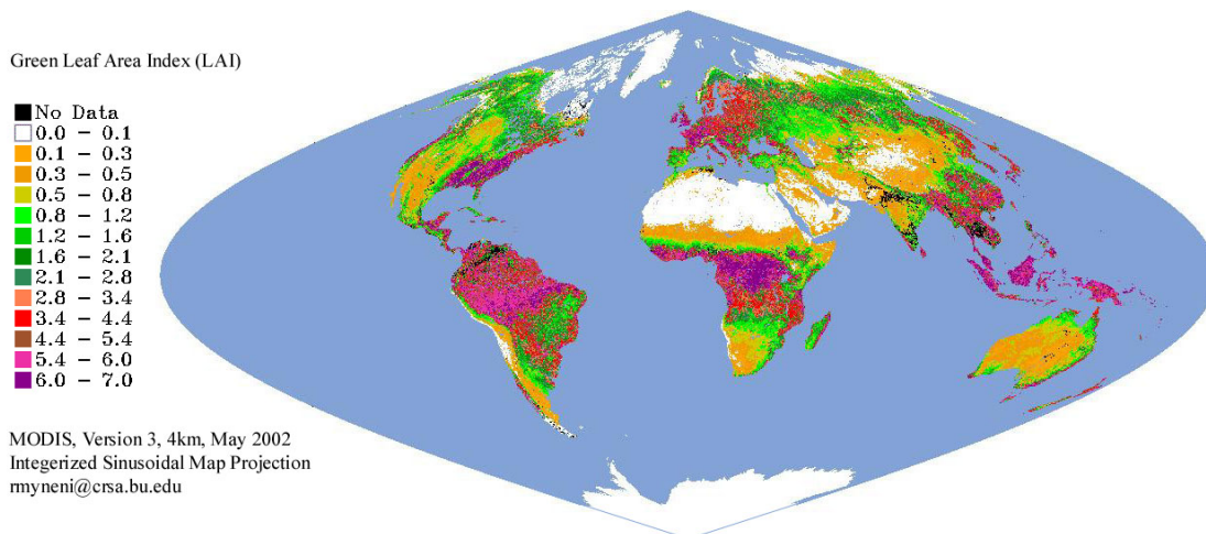
Figure 20 Global map of estimated leaf area index, May 2002. Lab of Ranga Myneni, Boston University.
