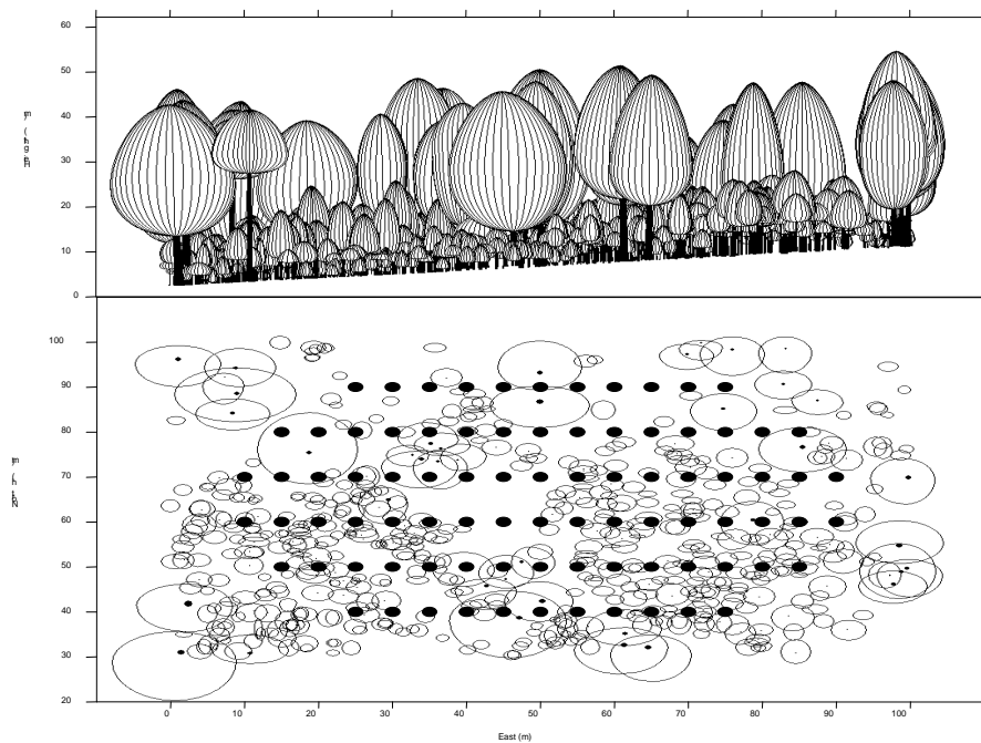
Figure 11 Spatial distribution of a ponderosa pine stand. (Law et al. , 2001).
