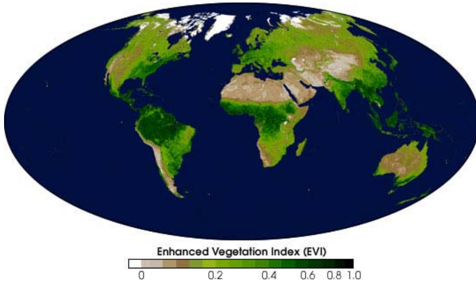
Figure 19 Global map of EVI. http://tbrs.arizona.edu:8080/modis/gm_index.htm
