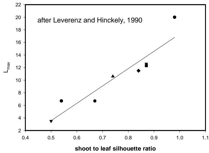
Figure 17 Comparison of maximum leaf area index the ratio between the projected shoot and needle area.
