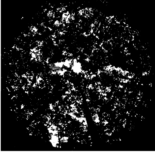
Figure 15 Hemispherical photograph of a deciduous, temperate broadleaved forest near Oak Ridge, TN.
