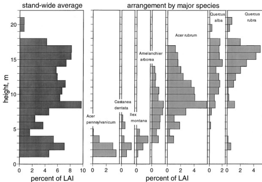
Figure 9 Profile of leaf area in an eastern deciduous forest. Parker GG, Brown MJ (2000)
