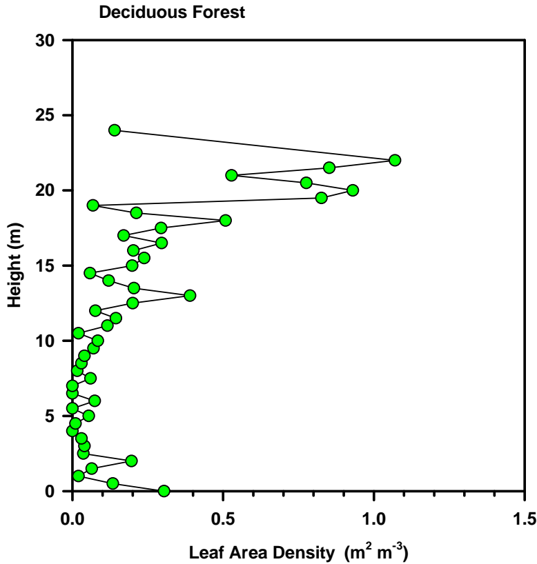
Figure 8 Leaf area profile, temperate broadleaved forest, Hutchison et al. (1986)
