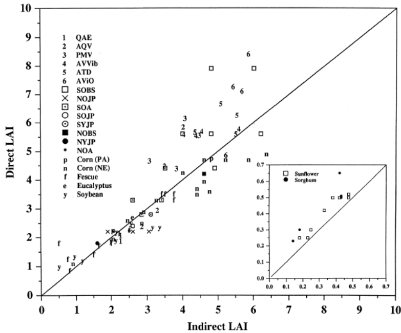
Figure 14 Test of estimates of leaf area index based on ‘direct’ allometric methods and ‘indirect’ light transmission methods. Gower et al, 1999
