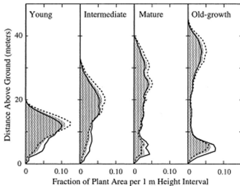
Figure 10 Variation of leaf area index profile with stand age, after (Harding et al. , 2001)
