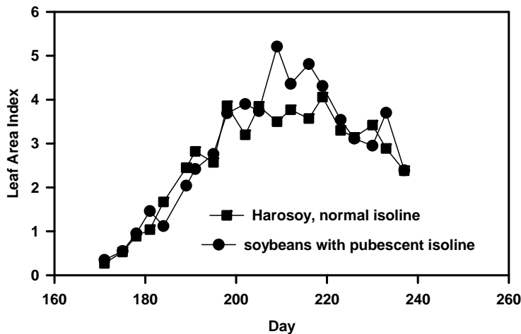
Figure 4 Seasonal variation of leaf area index of soybeans, growing near Mead, NE in 1979. data of D. Baldocchi.
