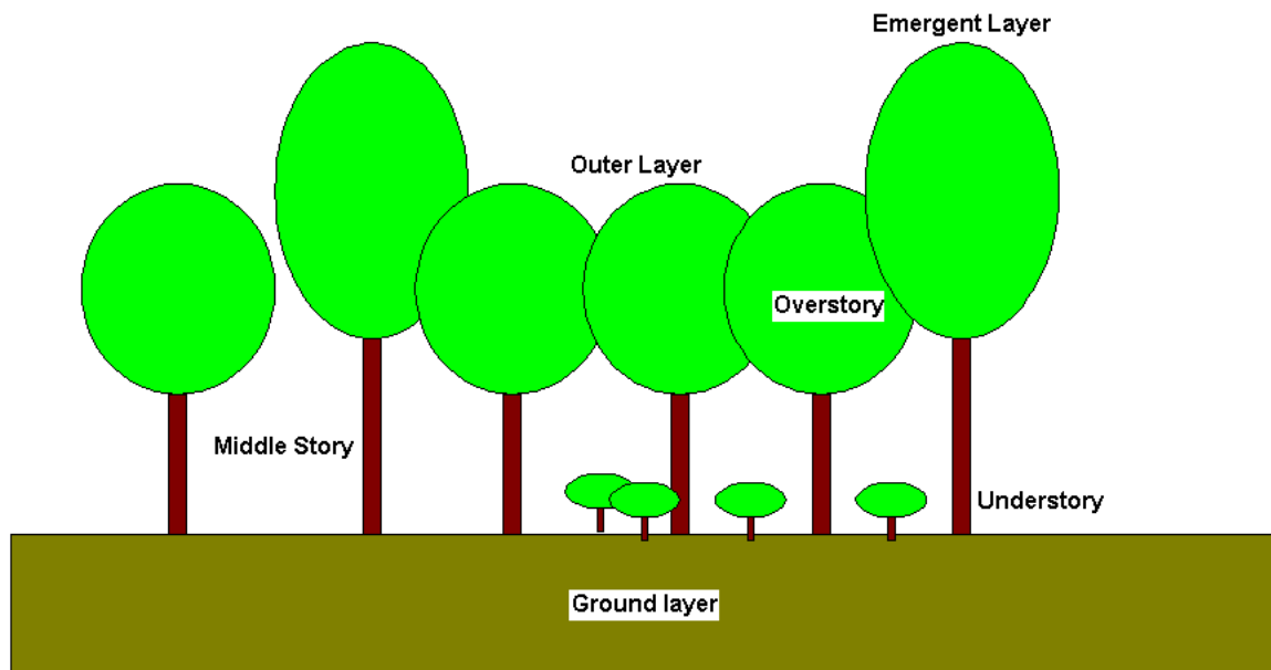
Figure 7 Schematic view of forest layers (adapted from Parker, 1995).
