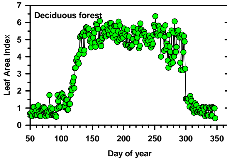
Figure 5 Seasonal change in leaf area index of a temperate broadleaf forest (Wilson, Baldocchi, 2000). Inferred from light transmission measurements.
