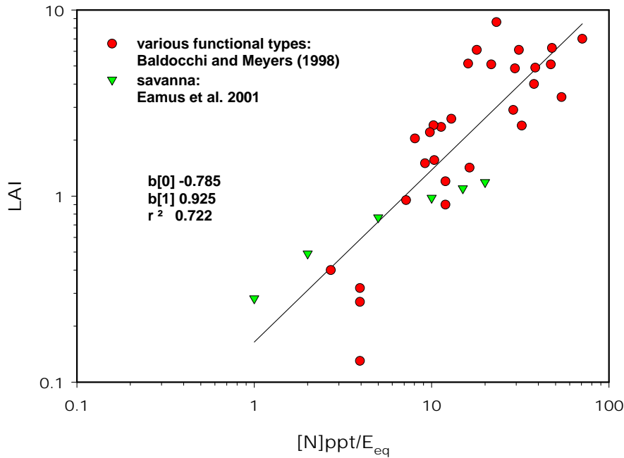
Figure 3 Correlation among leaf area index and climate and biogeochemical factors (precipitation, leaf nitrogen content and evaporation) (Baldocchi, Meyers, 1998; Eamus, Prior, 2001).
