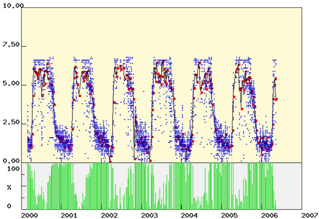
Figure 6 Seasonal variation in fraction of Leaf Area Index. These calculations were derived from MODIS sensor on the TERRA satellite. Data are available from the FLUXNET web site.
