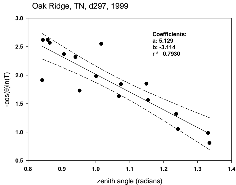
Figure 16 Relation between contact number and zenith angle, data of Baldocchi, Chason and Huston.
