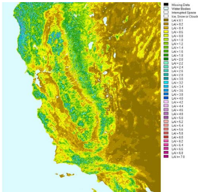
Figure 21 Summer maximum LAI in California. Computations by Ned Nikolov, 1 km resolution and corrected for clumping. Data are based on AVHRR data on the NOAA satellite (Nikolov, Zeller, 2006).
